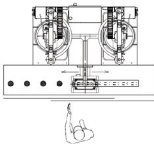
1) semi-automatic cell
