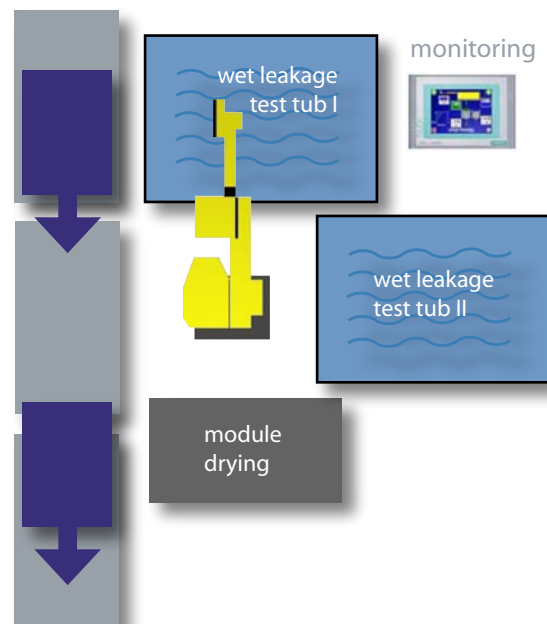
3) automated control setup with module drying (variable number of test tubs)
